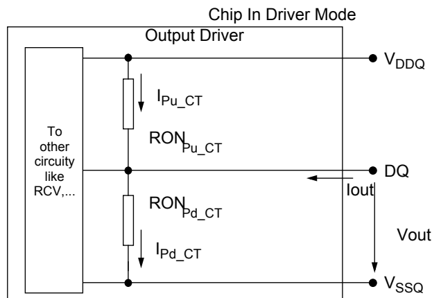
Figure 14. Output Driver
