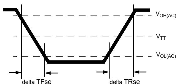
Figure 15. Single-ended Output Slew Rate Definition
