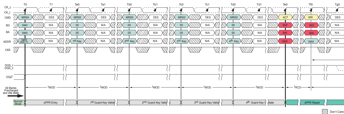
Figure 76: sPPR – Entry
