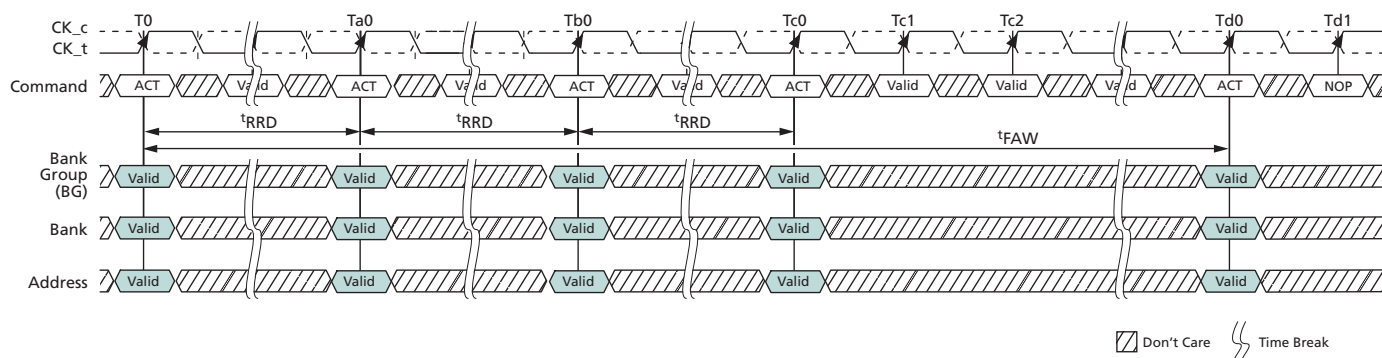
Figure 79: t_{FAW} Timing
