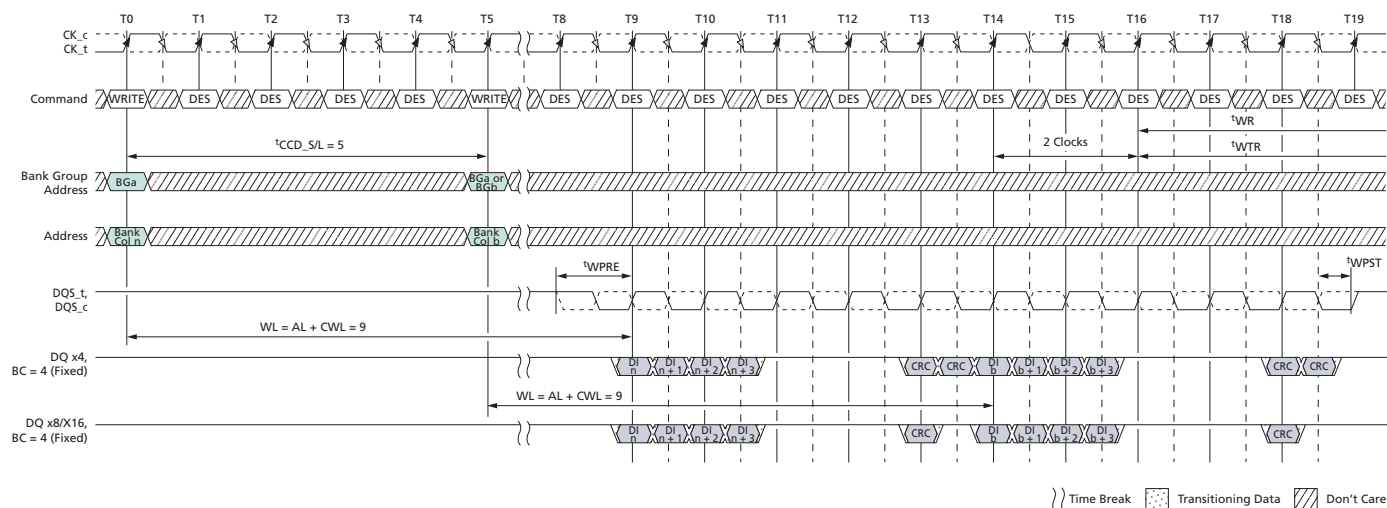
Figure 194: Consecutive WRITE (BC4-Fixed) with 1 st CK Preamble and Write CRC in Same or Different Bank Group
