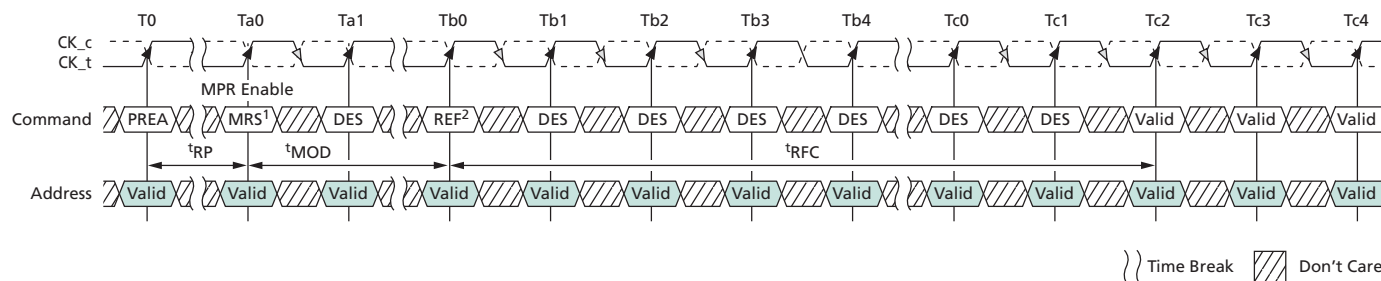
Figure 38: REFRESH Timing
