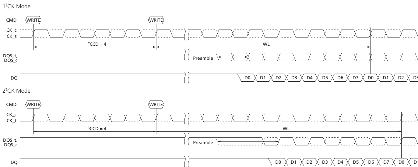
Figure 108: 1 t CK vs. 2 t CK WRITE Preamble Mode, t CCD = 4
